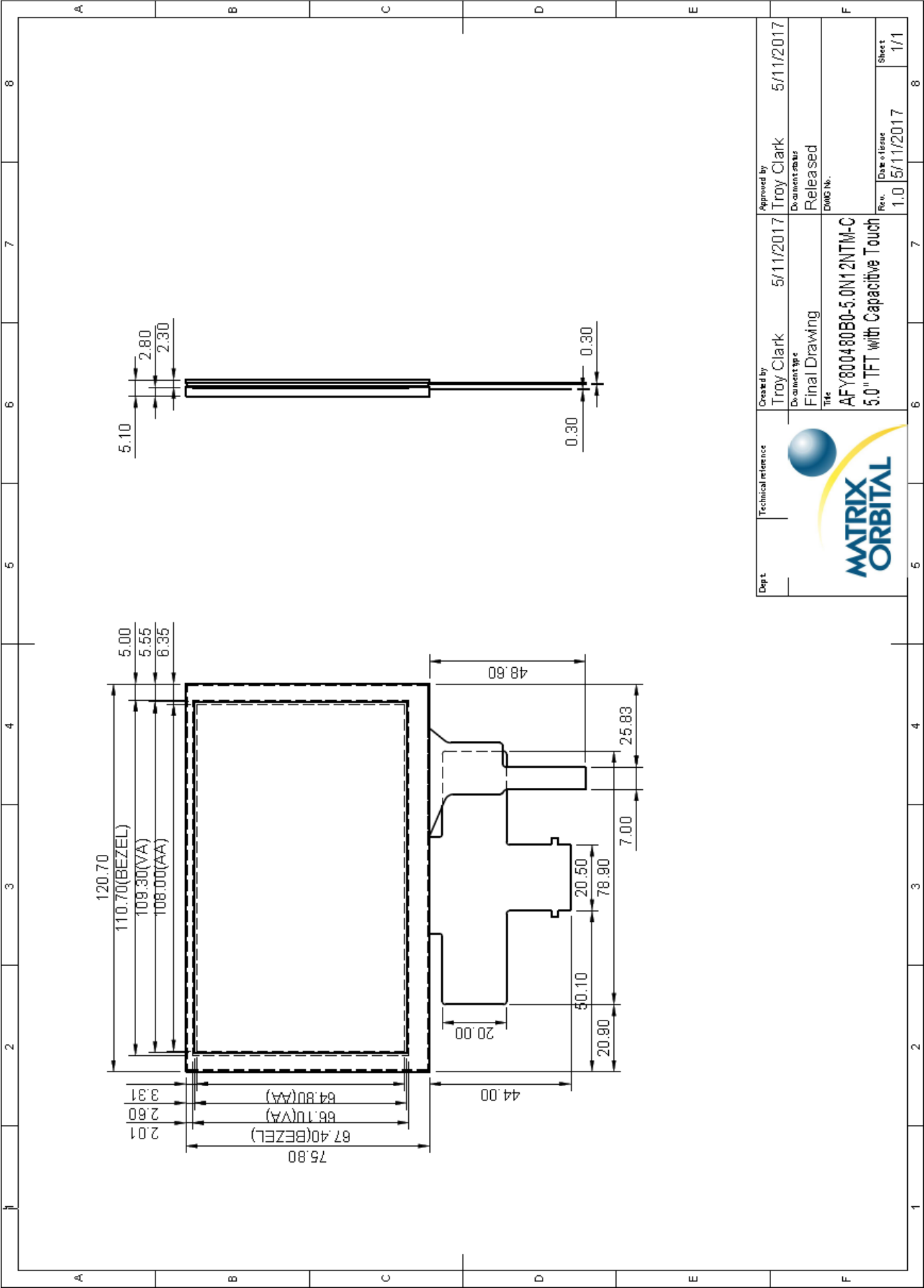
Figure 1: MOP-TFT800480-50A-BLM-TPC Drawing
